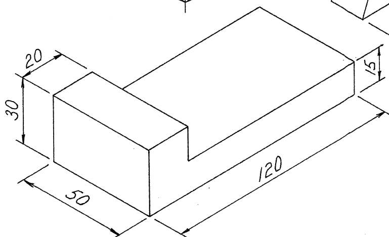
SEPARATED ISOMETRIC VIEW
