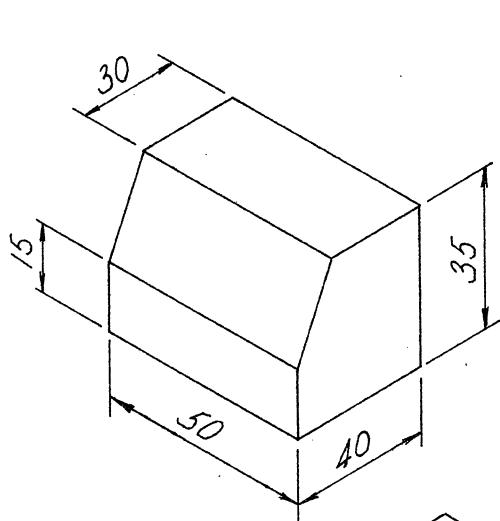
ISOMETRIC VIEW
