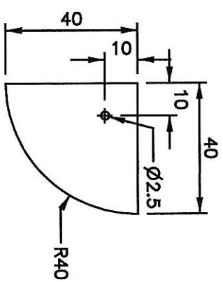
8 QUADRANT BLOCK PLASTIC
