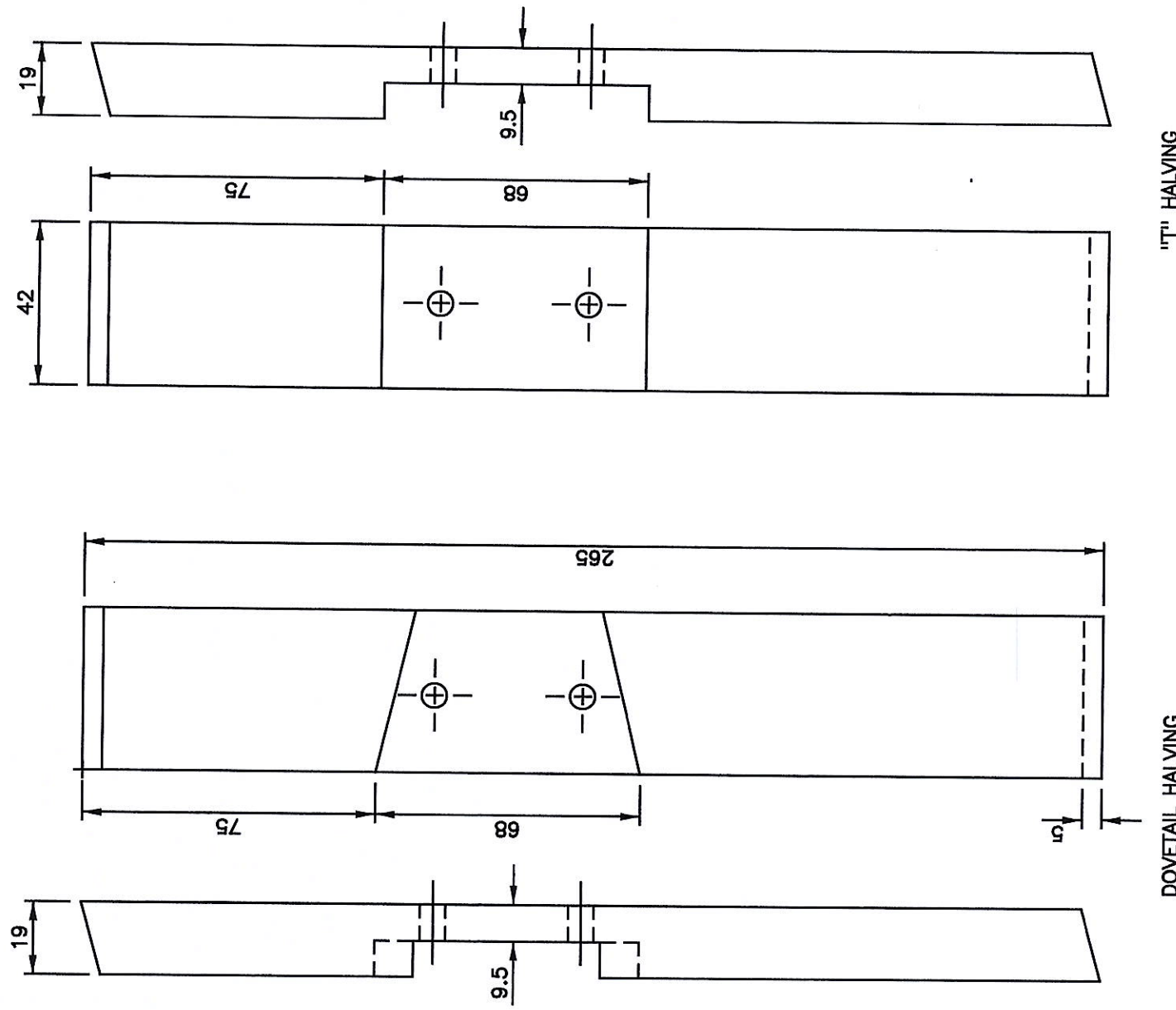
3 "H" FRAME LEG
