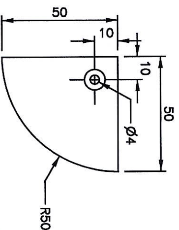
8 QUADRANT BLOCK PLASTIC
